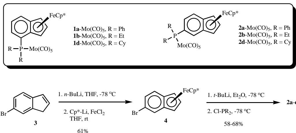
Scheme 1. Synthesis of benzoferrocenyl phosphine ligands 2a-e .
