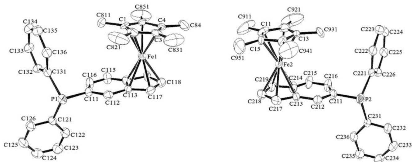
Fig. (1). ORTEP-3 drawing of the two major orientations of the molecules that constitute the asymmetric unit of 2a . Thermal ellipsoids are drawn at the 20% probability level. Selected bond distances and angles: Fe1-C1, 2.039(12)Å; Fe1-C2, 2.029(10)Å; Fe1-C3, 2.036(12)Å; Fe1-C4, 2.048(8)Å; Fe1-C5, 2.052(10)Å; Fe1-C113, 2.088(5)Å; Fe1-C114, 2.082(7)Å; Fe1-C117, 2.071(8) Å; Fe1-C118, 2.048(8)Å; Fe1-C119, 2.041(7)Å; P1-C131, 1.824(6) Å; P1-C111, 1.840(6)Å; P1-C121, 1.833(6)Å; C111-P1-C121, 101.4(3)°; C111-P1-C131, 100.0(3)°; C121-P1-C131, 103.5(3)°; Fe2-C11, 2.040(8)Å; Fe2-C12, 2.053(10)Å; Fe2-C13, 2.069(7)Å; Fe2-C14, 2.065(7)Å; Fe2-C15, 2.048(8)Å; Fe2-C213, 2.092(8)Å; Fe2-C214, 2.064(8)Å; Fe2-C217, 2.078(9)Å; Fe2-C218, 2.047(8)Å; Fe2-C219, 2.030(8)Å; P2-C211, 1.844(6)Å; P2-C221, 1.840(6)Å; P2-C231, 1.823(6)Å; C211-P2-C221, 99.8(3)°; C211-P2-C231, 102.2(3)°; C221-P2-C231, 102.3(3)°.
